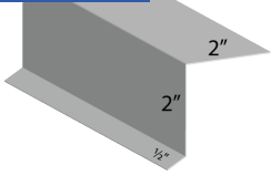
Eave
