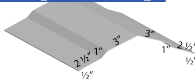
Sculptured Ridge
