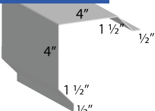
HP Corner
