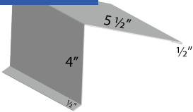
Peak
