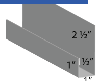
LP Header
