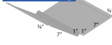
Valley
