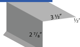
Corrugated Rake
