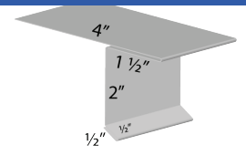
Zia Eave
